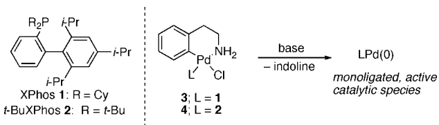
Figure 1. Formation of L 1 Pd(0) complexes bearing biarylphosphines.
